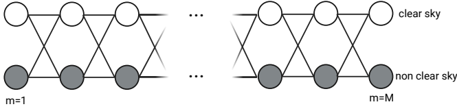
Fig. 4: A path from left to right corresponds to a clear sky estimate. Horizontal edges have no weight, and diagonal edges have weight \sigma . The nodes have weight zero or one, depending on the naïve clear sky value.
