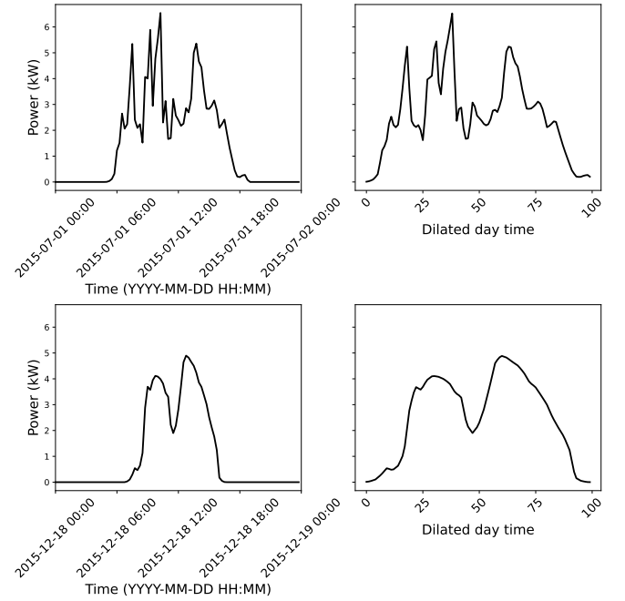
Fig. 7: Time dilation of PV output. Top . Summer. Bottom . Winter.
