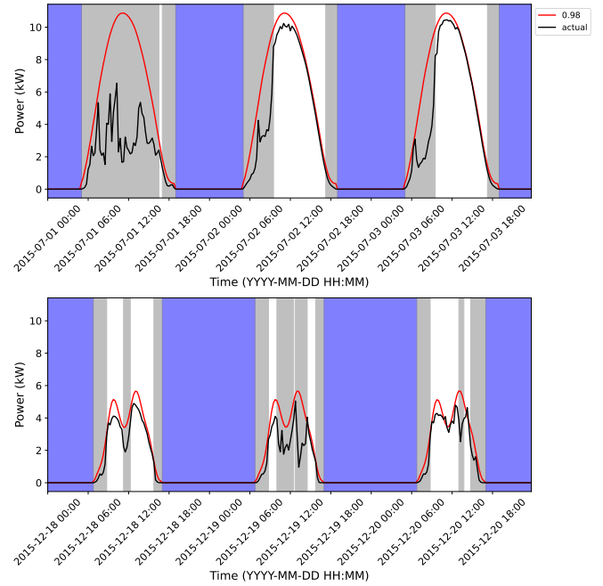
Fig. 9: Detected clear sky time intervals. Top . Summer. Bottom . Winter.
