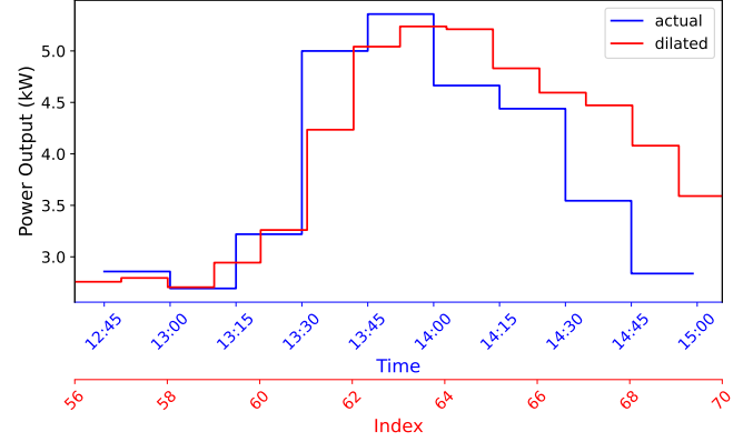
Fig. 3: Actual signal and time dilated signal corresponding to the same time interval.
